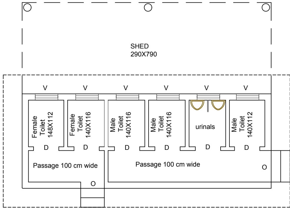
PLAN OF EXISTING TOILET BLOCK BEHIND L/C PLANT
