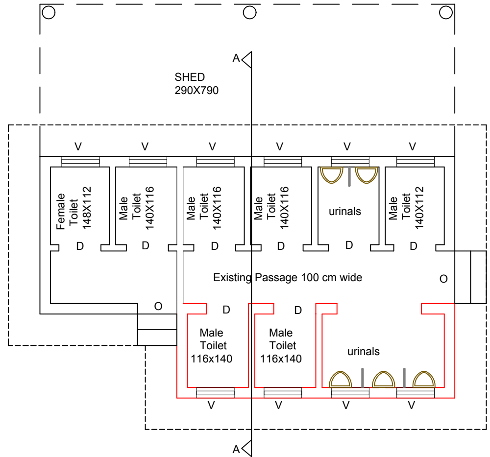
PLAN OF PROPOSED EXTENSION OF TOILET BLOCK BEHIND L/C PLANT-Option-2
