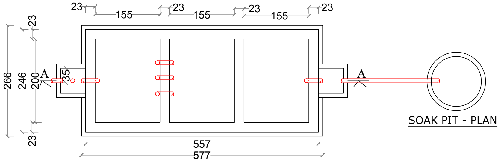
SEPTIC TANK - PLAN
