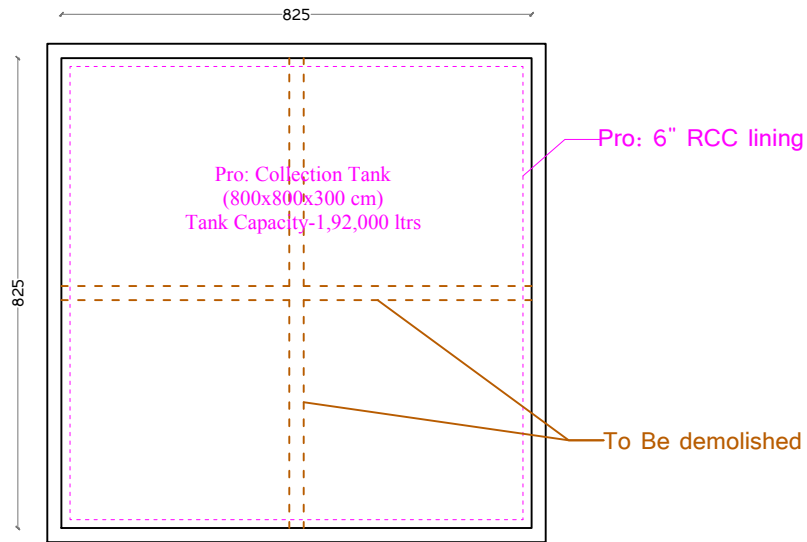
PLAN Pro: Collection Tank (800x800x300 cm) Tank Capacity-1,92,000 ltrs
