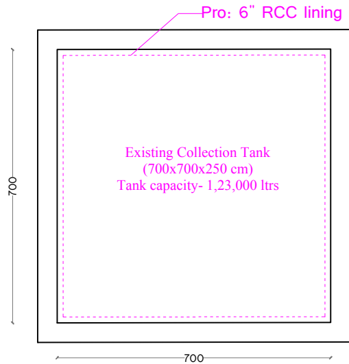
PLAN Existing Collection Tank (700x700x250 cm) Tank capacity- 1,23,000 ltrs
